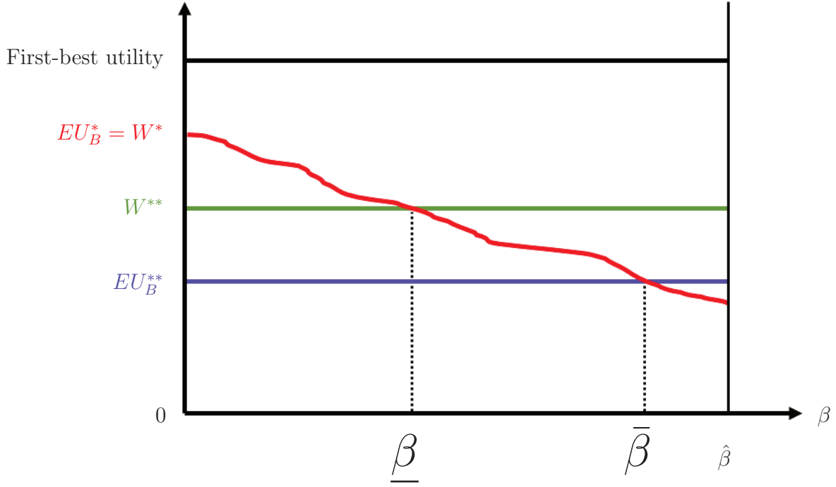
Figure 2: Illustration of Proposition 4.
