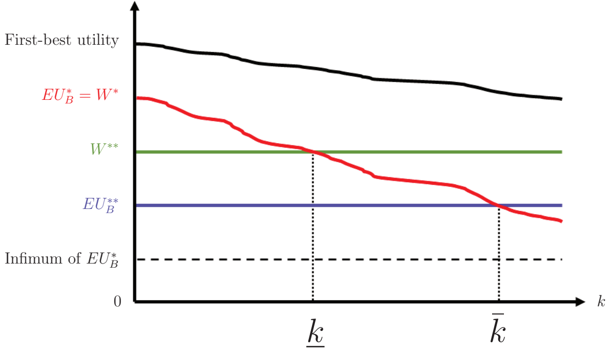
Figure 1: Illustration of Proposition 3.
